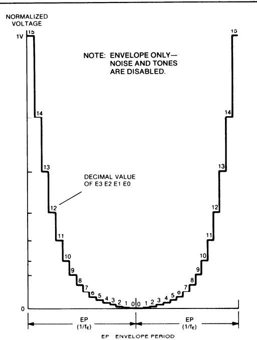
Fig. 3 D/A CONVERTER OUTPUT
