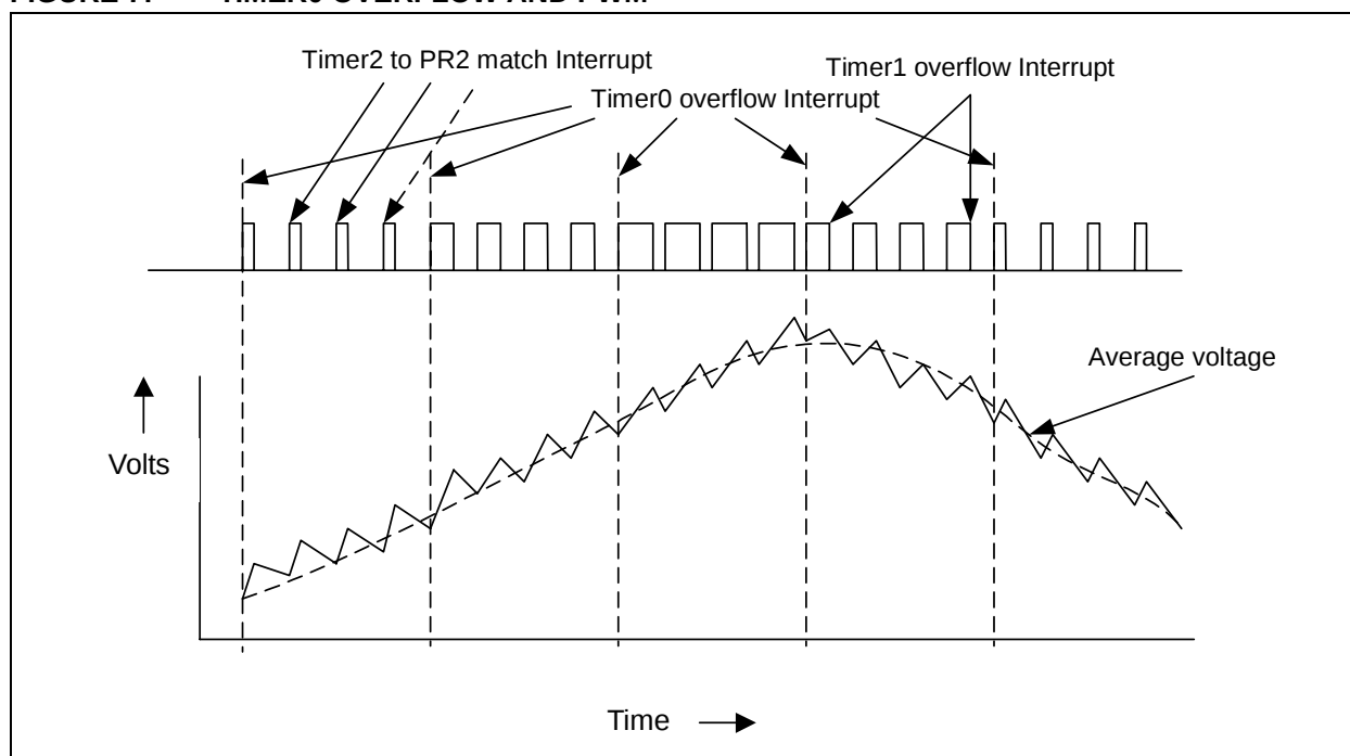
FIGURE 7: TIMER0 OVERFLOW AND PWM
