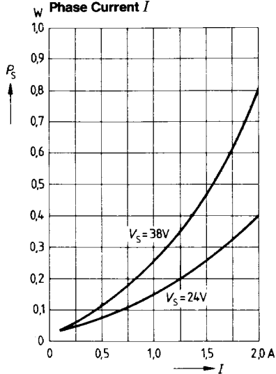
Switching Loss P_{\text{S}} versus Phase Current I
