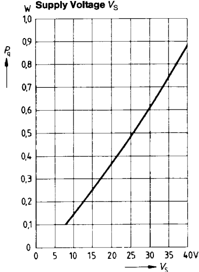
Quiescent Current Loss P_{\text{q}} versus Supply Voltage V_S
