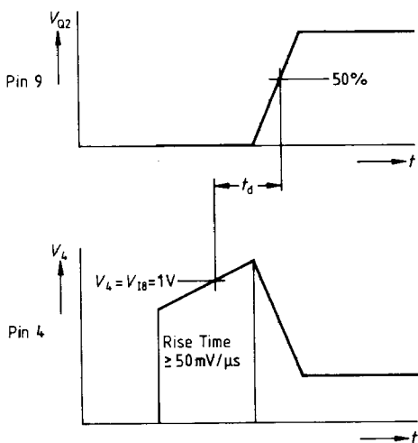
Figure 4 Turn-OFF Delay
